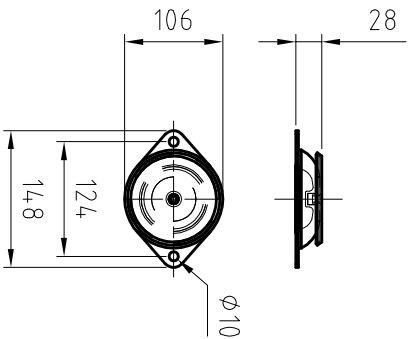
NR. 8 RUBBER ANTIVIBRATION MOUNTS TYPE CAPK 100-60
